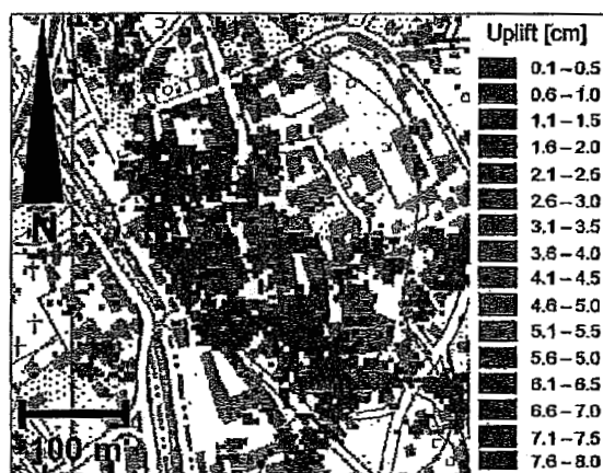
Fig. 15: Analysis of satellite-based ground level uplift monitoring by radar interferometry, a) July 2008 to 29. October 2008, b) July 2008 to 3. January 2009, c) July 2008 to 25. January 2009.
