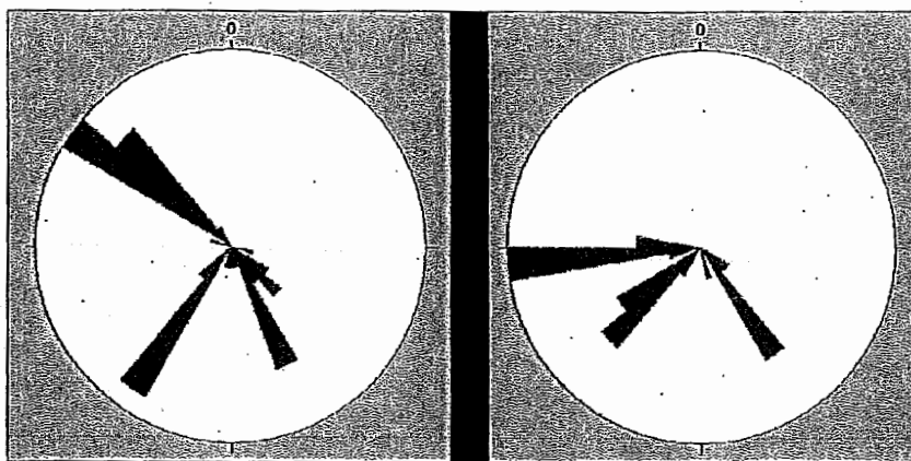
Fig. 19: Rose diagrams of outcrops.
