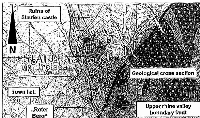
Fig. 6: Modified detail image of the geological map of Freiburg, M 1:50.000. (Landesvermessungsamt Baden-Württemberg 1996).
