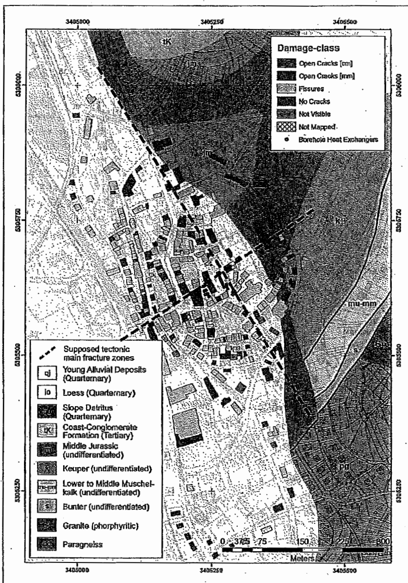
Fig. 18: Mapping of damages and geology.
